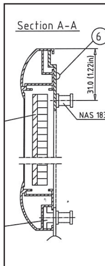
PNR 1380-series • frame section
